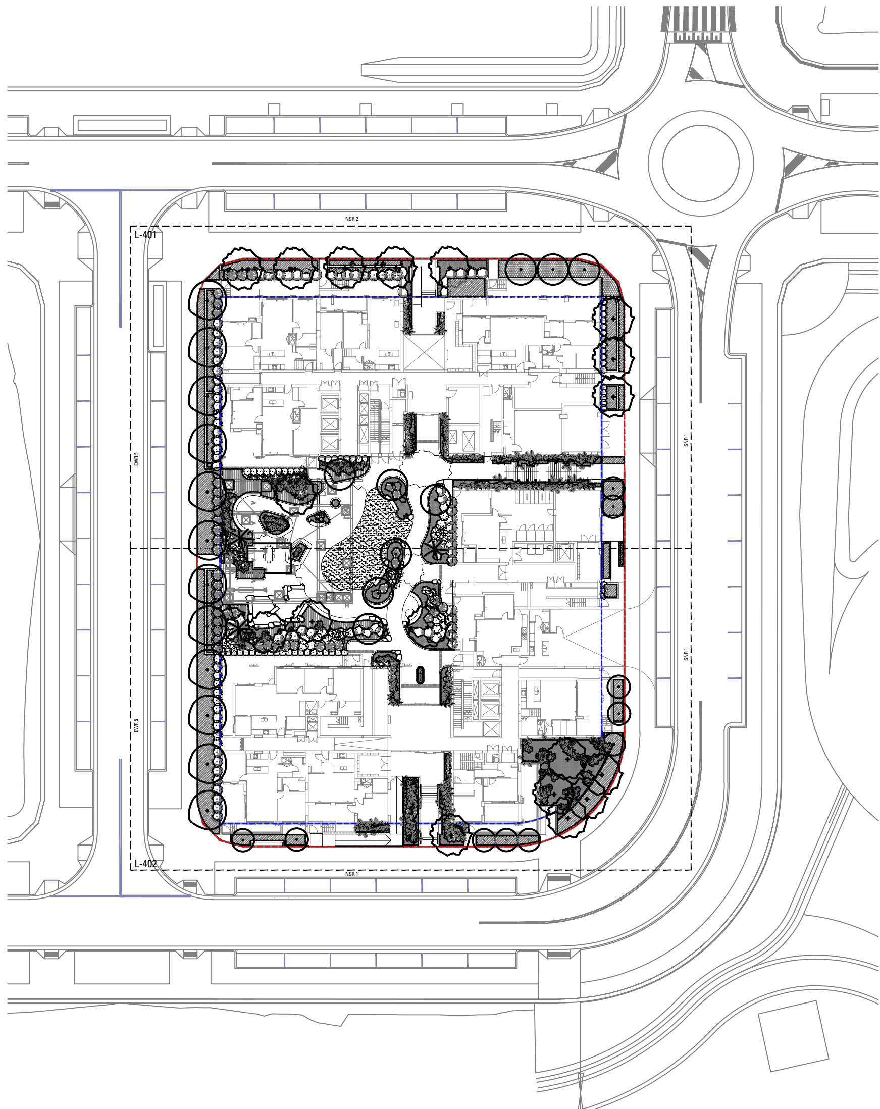
GROUND FLOOR
